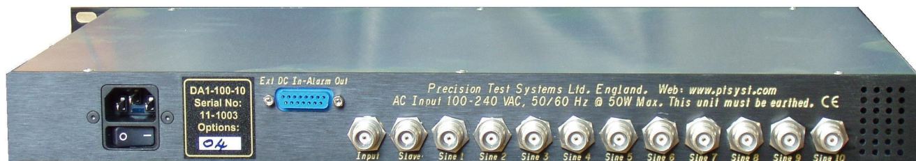
DA1-100-10-150MHz Rear view (with option 04 TNC Connectors).
